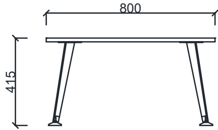
MT5080S -MIO SEHPA 50X80
