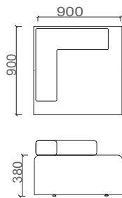
BRK1129 Bend Arm Ottoman
