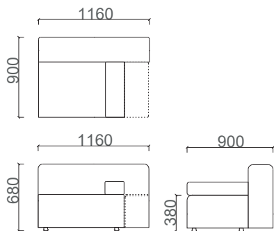
BRK1125 Bend Corner Waiting with Table 110 Left
