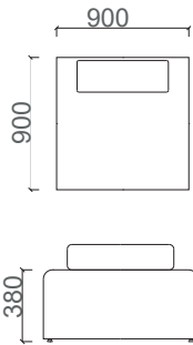
BRK1130 Bend L Arm Ottoman
