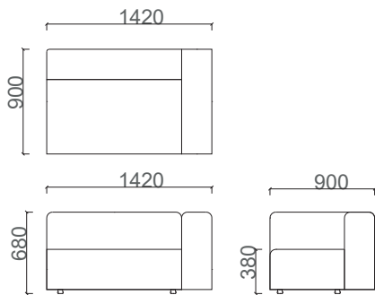
BRK1123 Bend Corner Waiting 140 Left
