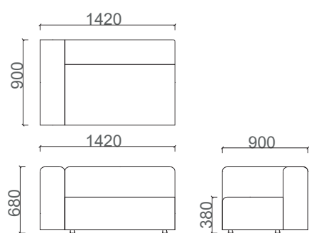
BRK1122 Bend Corner Waiting 140 Right
