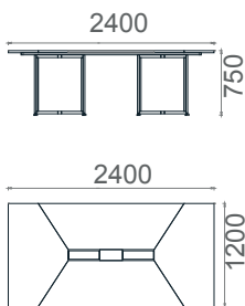
MLT120240 Mila Meeting Table 120x240
