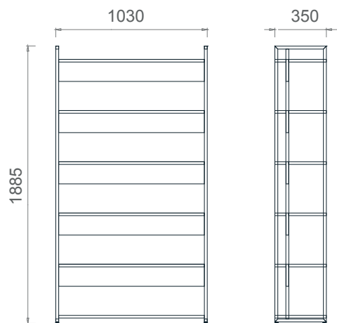
MK103190 MILA WORKBOOK - 103x35x190h
