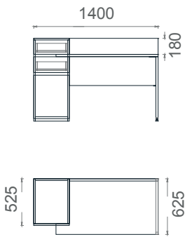
MDO60140 Mila Home Office Desk Left Cabinet 60x140
