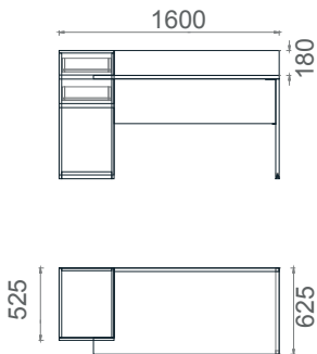
MDO60160 Mila Home Office Desk Left Cabinet 60x160
