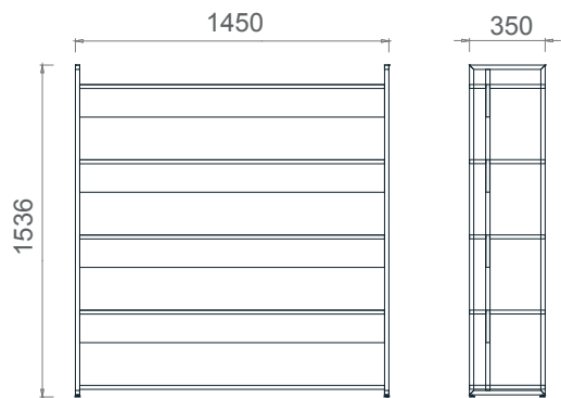
MKK14135 MILA WORKBOOK 142x35x154h
