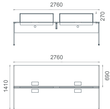
MLM70140W4 Mila Quad Workstation 70x140
