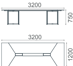
MLT120320 Mila Meeting Table 120x320
