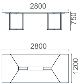
MLT120280 Mila Meeting Table 120x280
