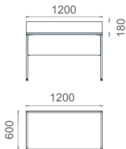
MTS60120 Mila Home Office Desk 60x120
