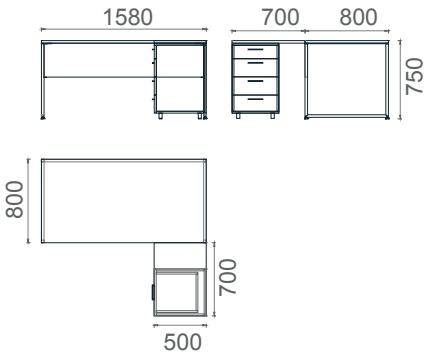
MLM80160 Mila L Work Desk 80x160
