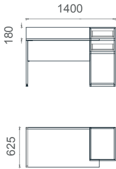
MDS60140 Mila Home Office Desk Right Cabinet 60x140
