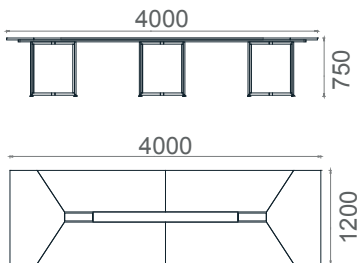
MLT120400 Mila Meeting Table 120x400
