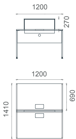
MLM70120W2 Mila Dual Workstation 70x120
