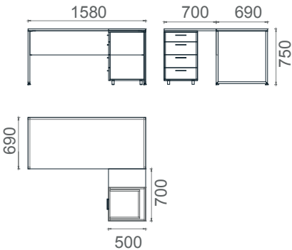
MLM70160 Mila L Work Desk 70x160
