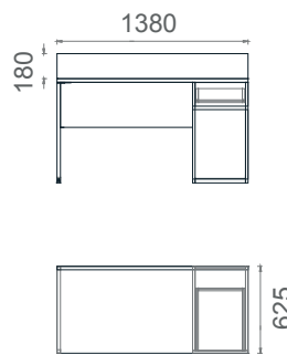
MKA60140 Mila Home Office Desk Right Drawer 60x140
