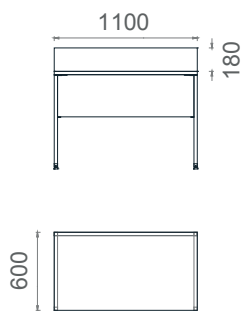
MTS60110 Mila Home Office Desk 60x110
