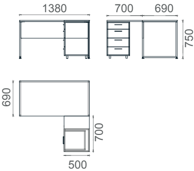
MLM70140 Mila L Work Desk 70x140
