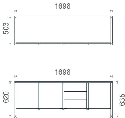
MLA50170 Mila Right Long Credenza 170x50x64h
