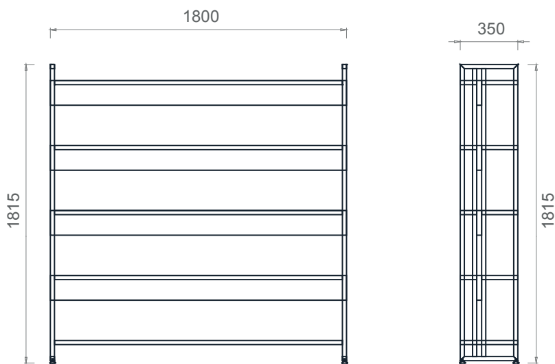
MYK18035 Mila Executive Bookshelf 180x35x182h
