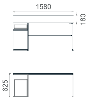
MKO60160 Mila Home Office Desk Left Drawer 60x160
