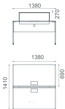
MLM70140W2 Mila Dual Workstation 70x140
