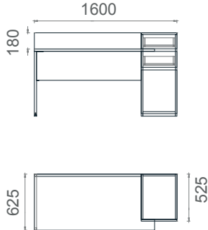
MDS60160 Mila Home Office Desk Right Cabinet 60x160
